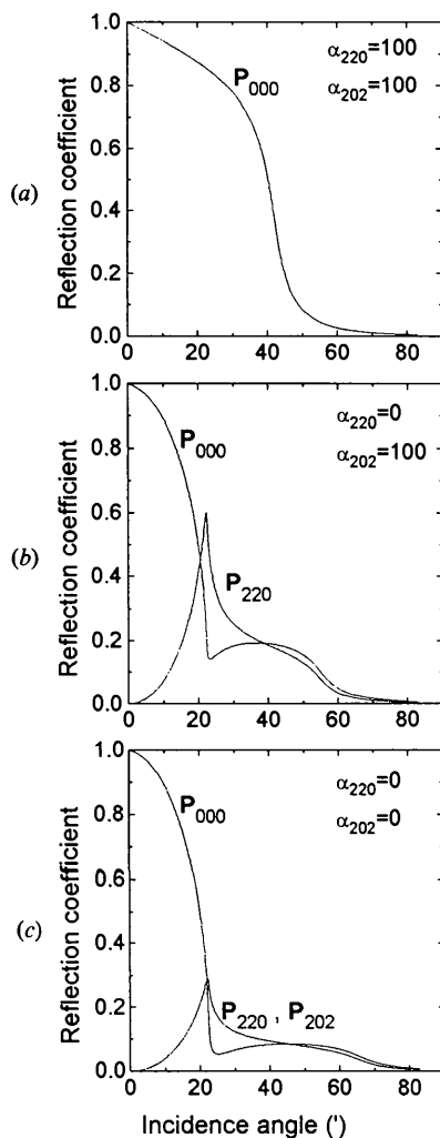
Fig. 2. Rocking curves of three-beam grazing-incidence diffraction 000, 220, 202 in germanium.
