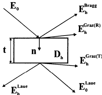
Fig. 1. Schematic presentation of X-ray multiple diffraction in a crystal plate.
